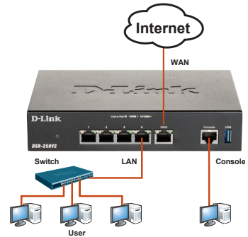
Figure 3. Basic Cabling Example
