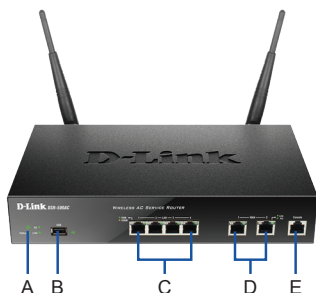
Figura 1. Panel Frontal DSR-500AC/1000AC
