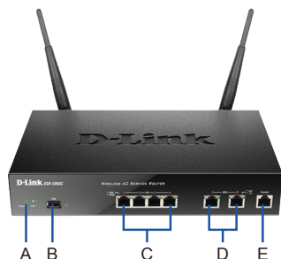
Figura 1. Painel Frontal do DSR-500AC/1000AC
