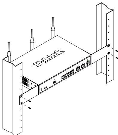
Gambar 4. Memasang Wireless AC Services Router ke rak peralatan ukuran standar.
