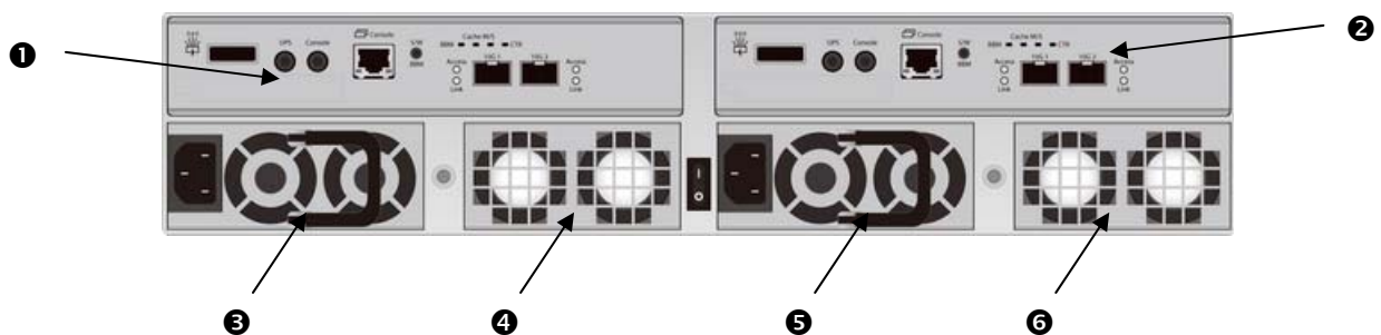
Figure 2.3.4.1 (DSN-6420 SFP+)
