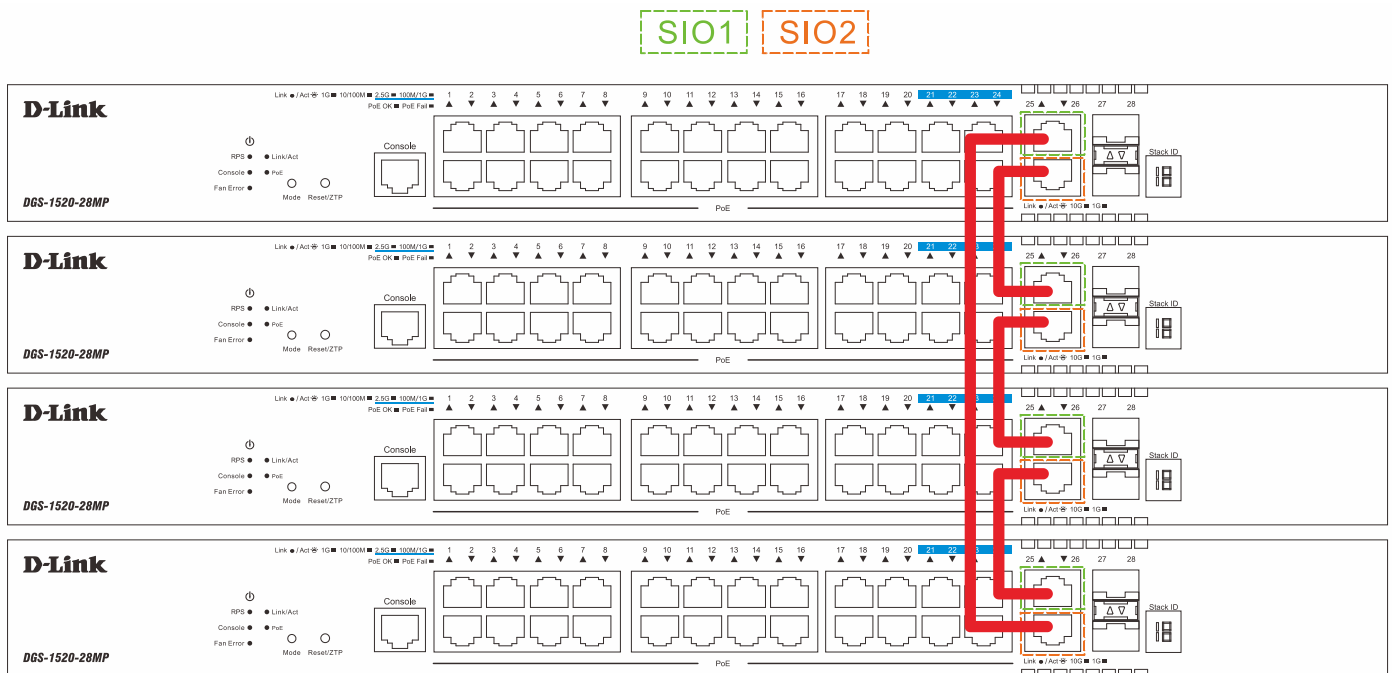
Figure 4-2 Duplex Ring Stacking Topology (Even, 2-port)
