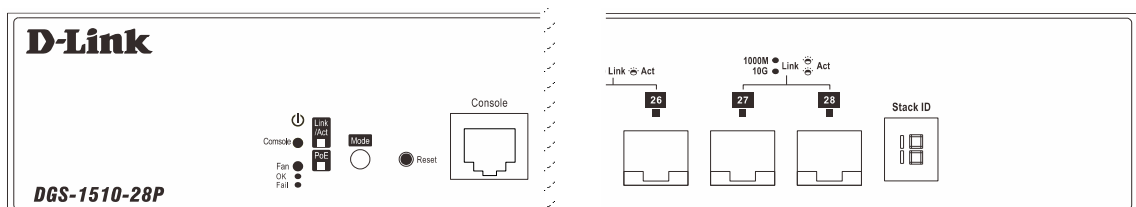
Figure 1-10 LED indicators for a DGS-1510-28P Switch
