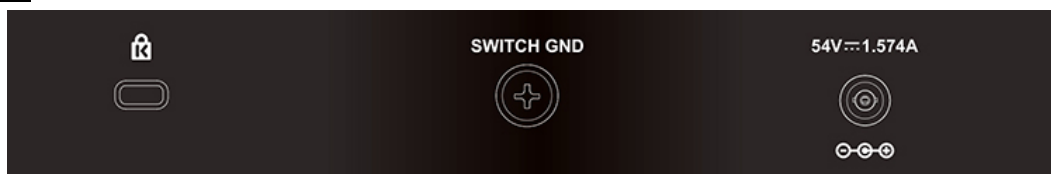
Figure 1.8 – DGS-1100-08P Rear Panel
