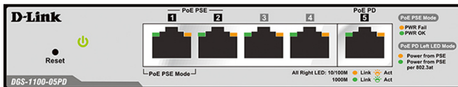
Figure 1.3 – DGS-1100-05PD Front Panel
