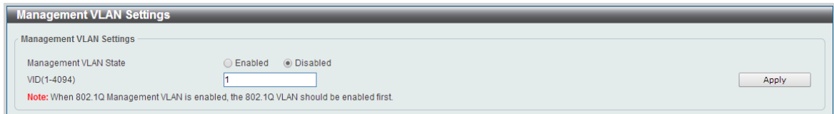
Figure 8-8 Asymmetric VLAN window
