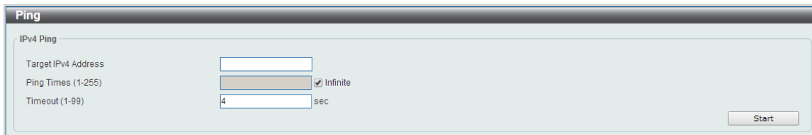
Figure 15-13 Ping window
