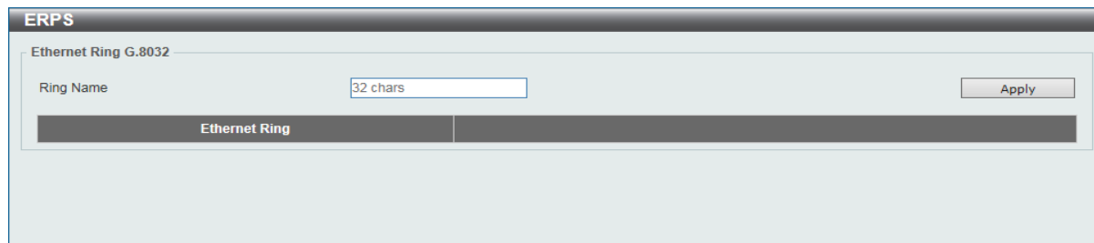
Figure 8-27 ERPS window
