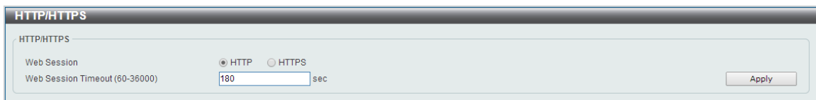
Figure 7-5 HTTP/HTTPS window
