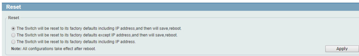
Figure 15-15 Reset window
