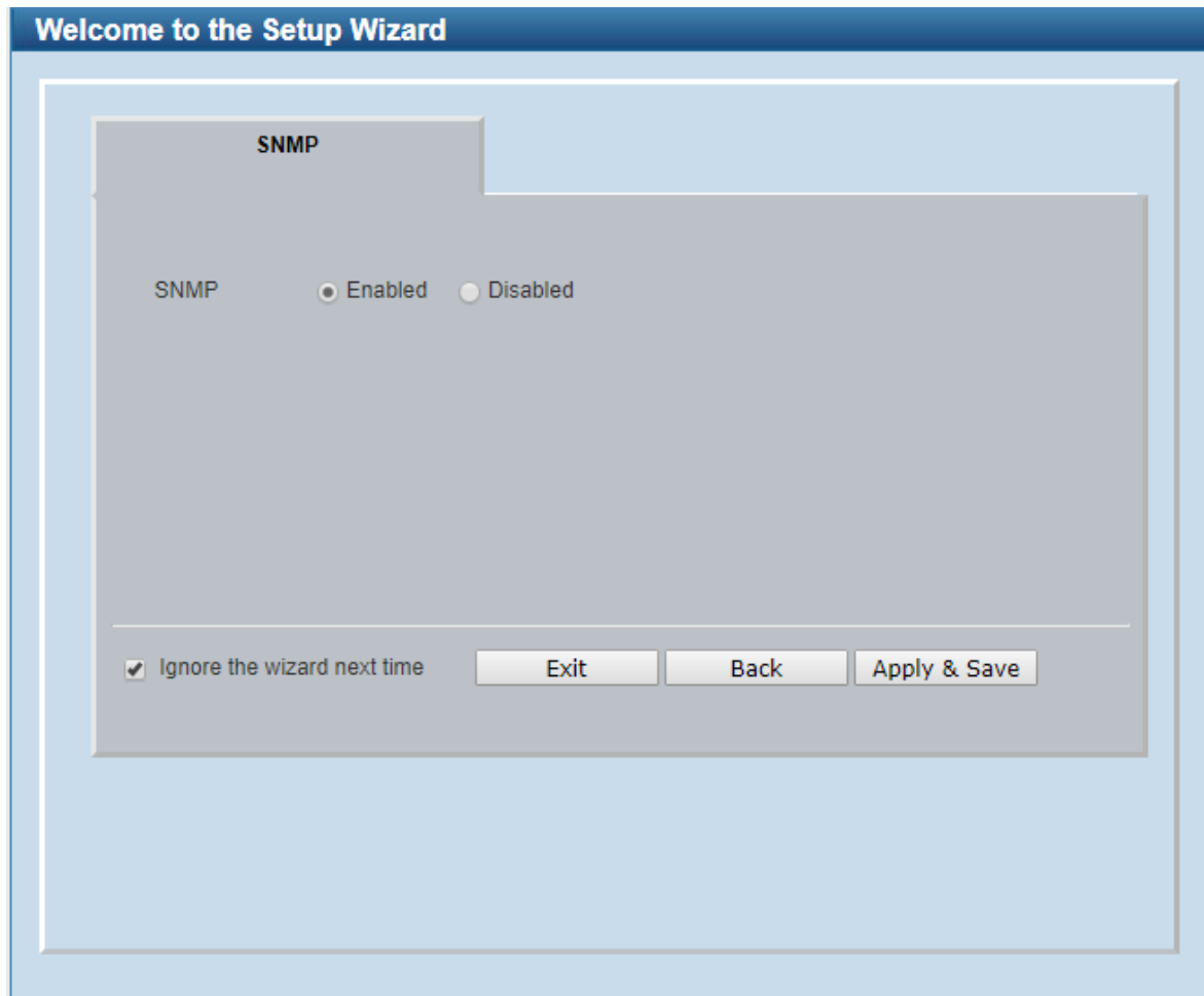
Figure 4-4 SNMP window
