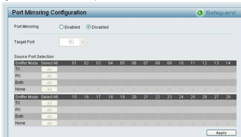
Figure 49 – Configuration > Port Mirroring
