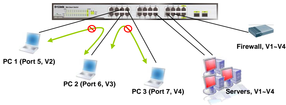
Figure 49 – Configuration > 802.1Q VLAN > Asymmetric VLAN Example
