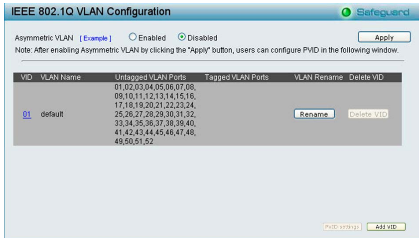
Figure 45 – Configuration > 802.1Q VLAN > Default Setting
