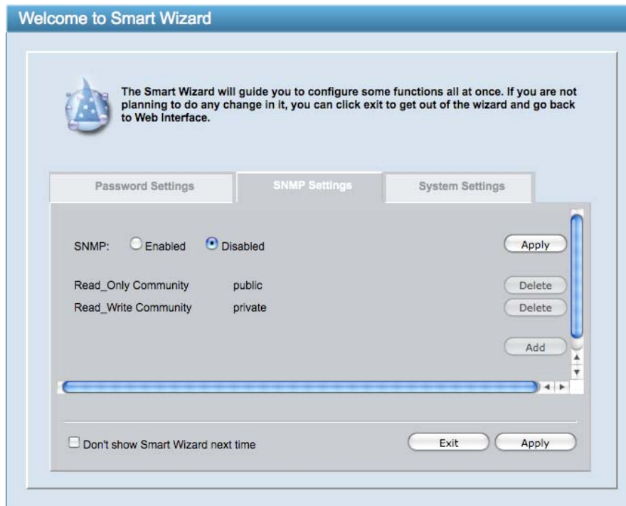
Figure 26 – Configure SNMP in Smart Wizard
