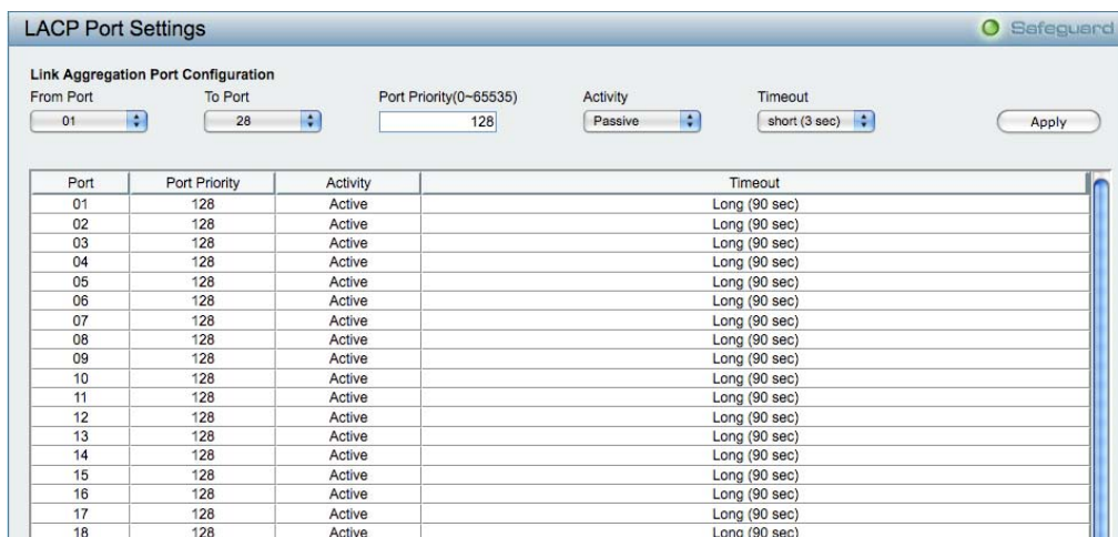
Figure 53 – Configuration > Link Aggregation > LACP Port Settings
