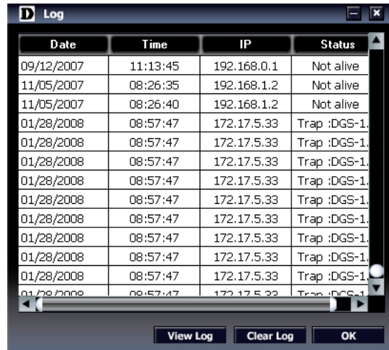
Figure 14 – SmartConsole Log
