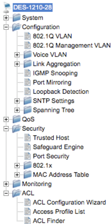
Figure 40 –Function Tree
