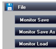
Figure 16 – SmartConsole File
