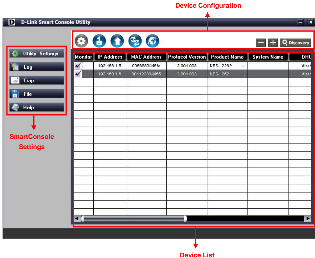
Figure 12 – SmartConsole Utility
