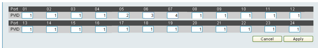
Figure 42 – Configuration > 802.1Q VLAN > Asymmetric VLAN – Assign PVID
