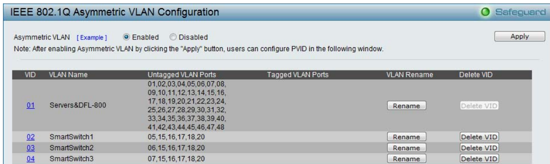
Figure 41 – Configuration > 802.1Q VLAN > Asymmetric VLAN – Create VLANs
