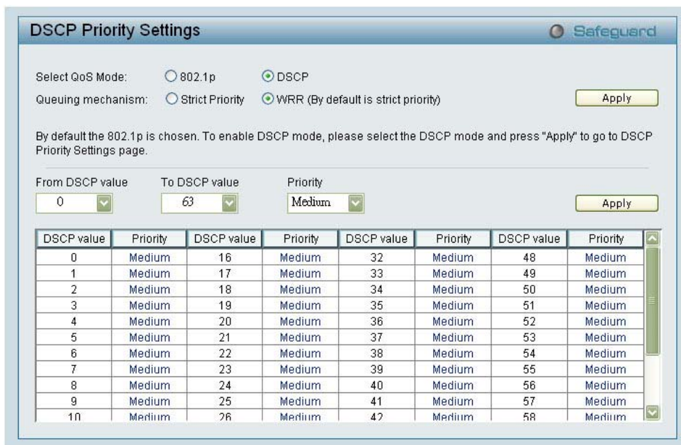
Figure 55 – QoS > DSCP Priority Settings
