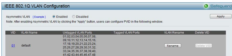
Figure 50 – Configuration > 802.1Q VLAN > Asymmetric VLAN - Enabling Asymmetric VLAN
