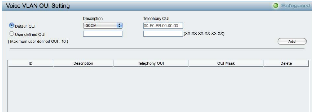
Figure 45 – Configuration > Voice VLAN > Voice VLAN OUI Setting
