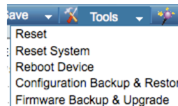
Figure 33 – Tool Menu
