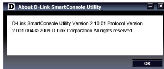
Figure 17 – SmartConsole Help
