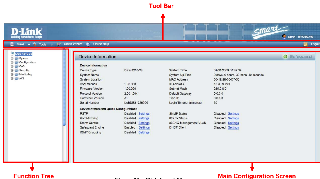
Figure 29 – Web-based Management
