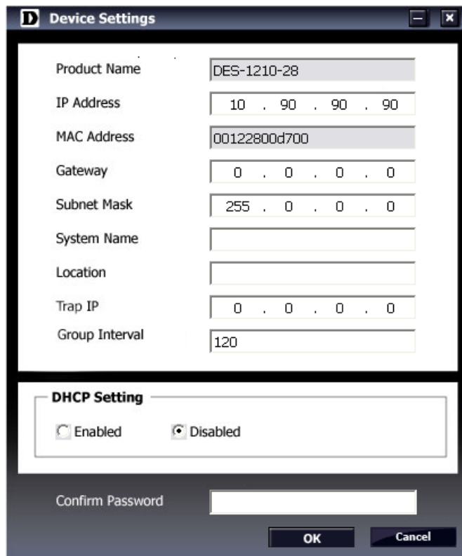
Figure 18 – SmartConsole Device Settings
