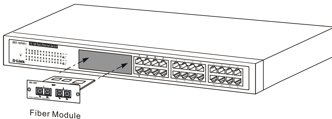
Figure 2.5 Sliding the module into position
