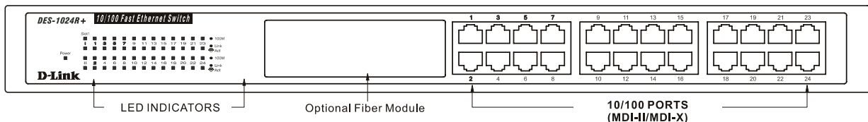
Figure 3.1 Front panel view of the DES-1024R+ Switch
