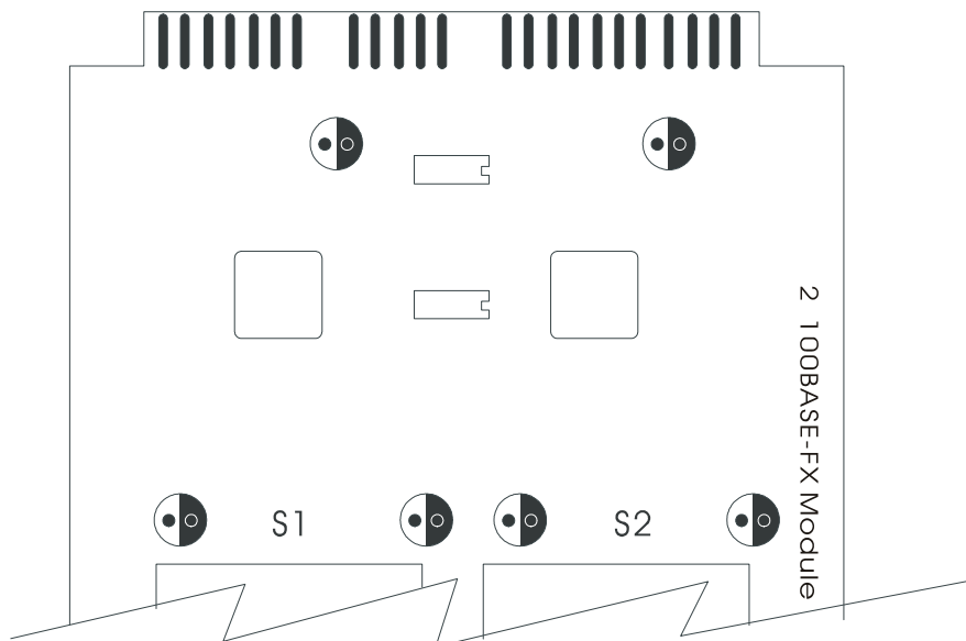
Figure 2.3 Jumper settings on the module
