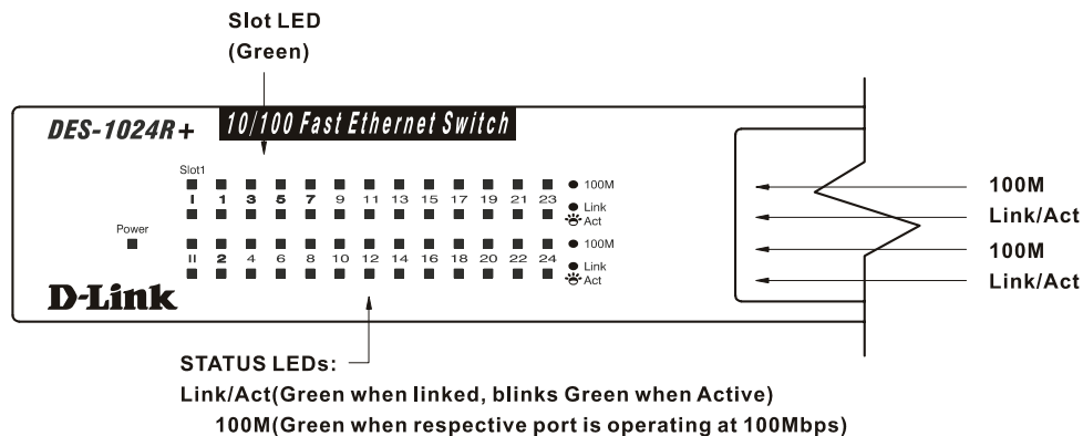
Figure 3.3 The DES-1024R+ Switch LED indicators
