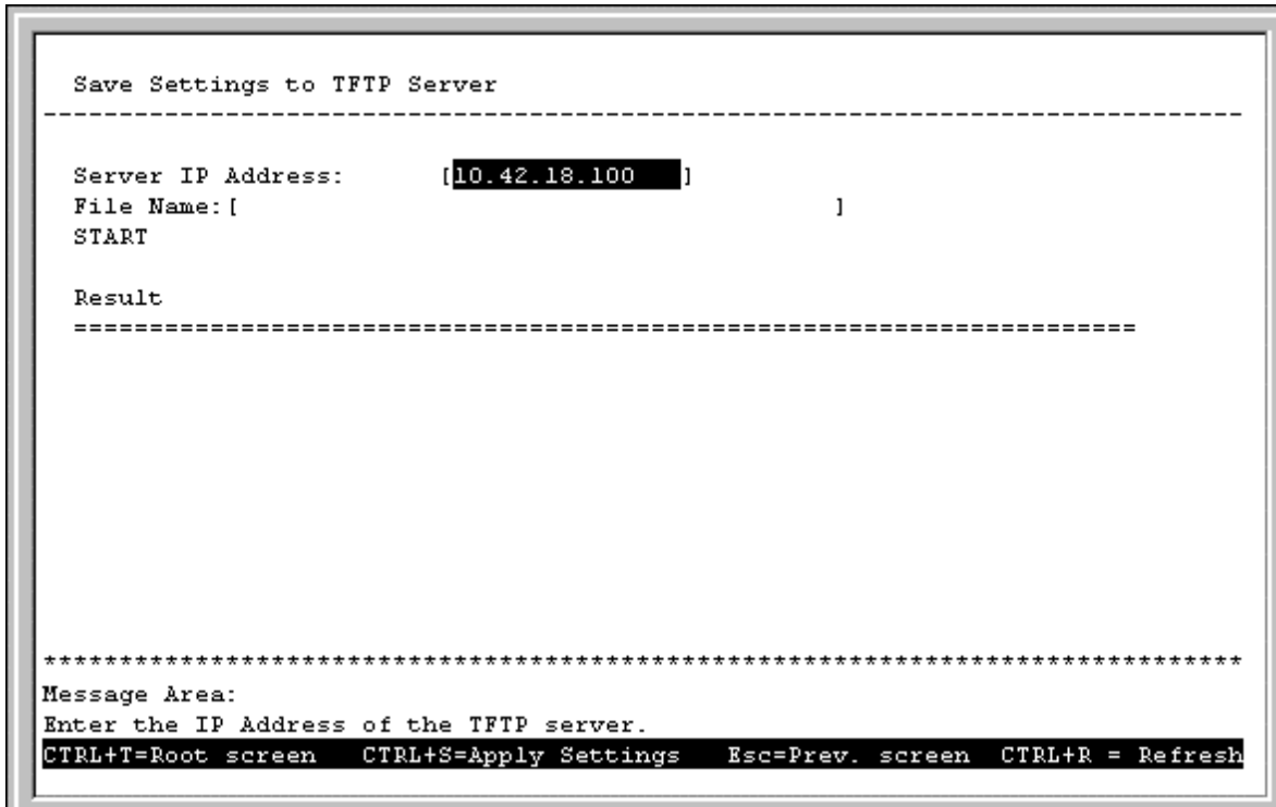
Figure 6-49. Save Settings to TFTP Server screen
