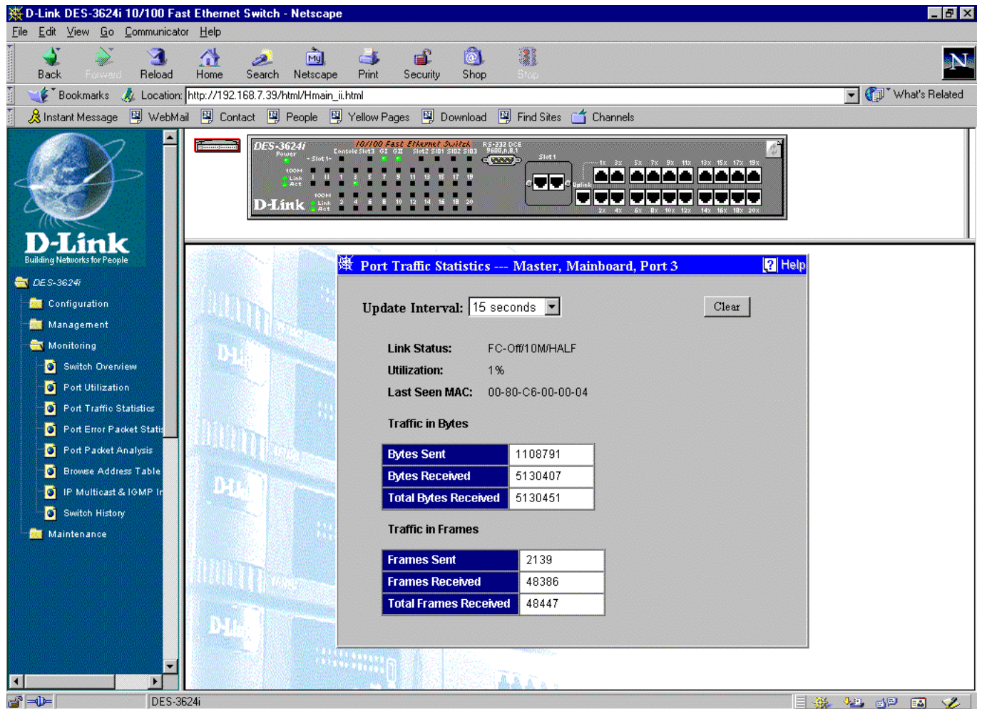
Figure 7-44. Port Traffic Statistics window
