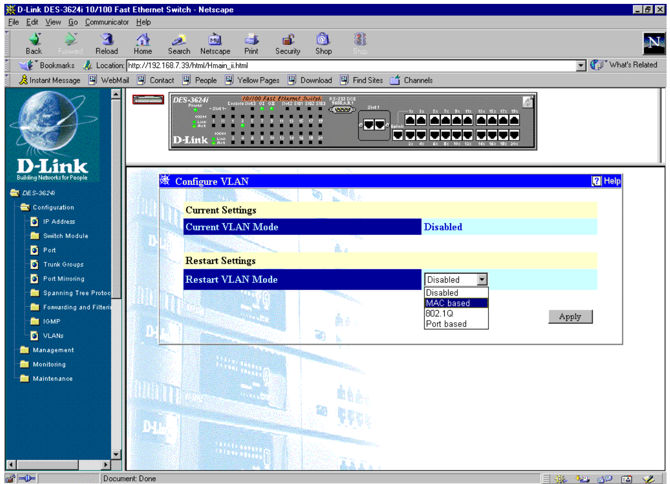
Figure 7-22. Configure VLAN window
