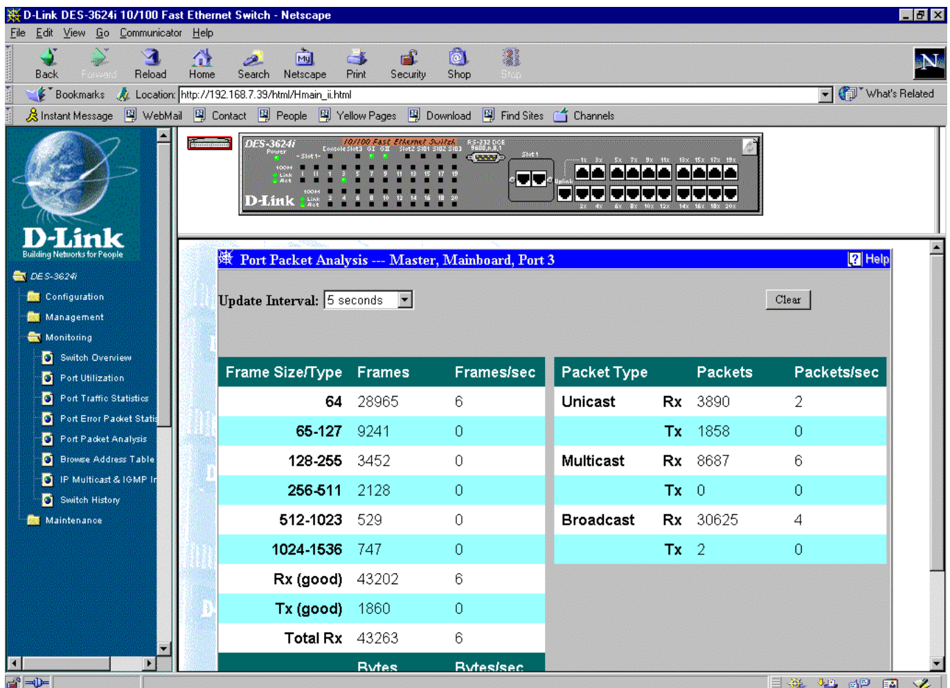
Figure 7-46. Port Packet Analysis window
