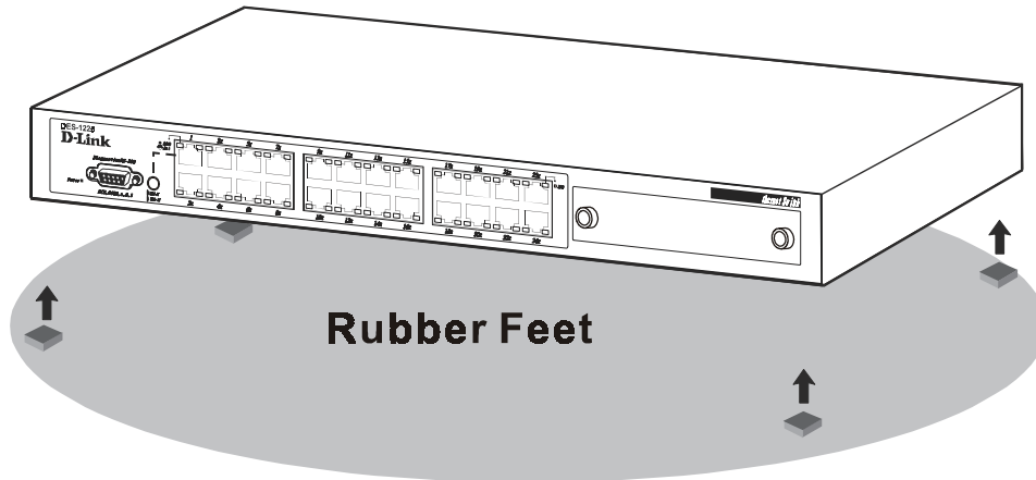
Figure 2-1 DES-1226 Switch installed on a Desktop or Shelf
