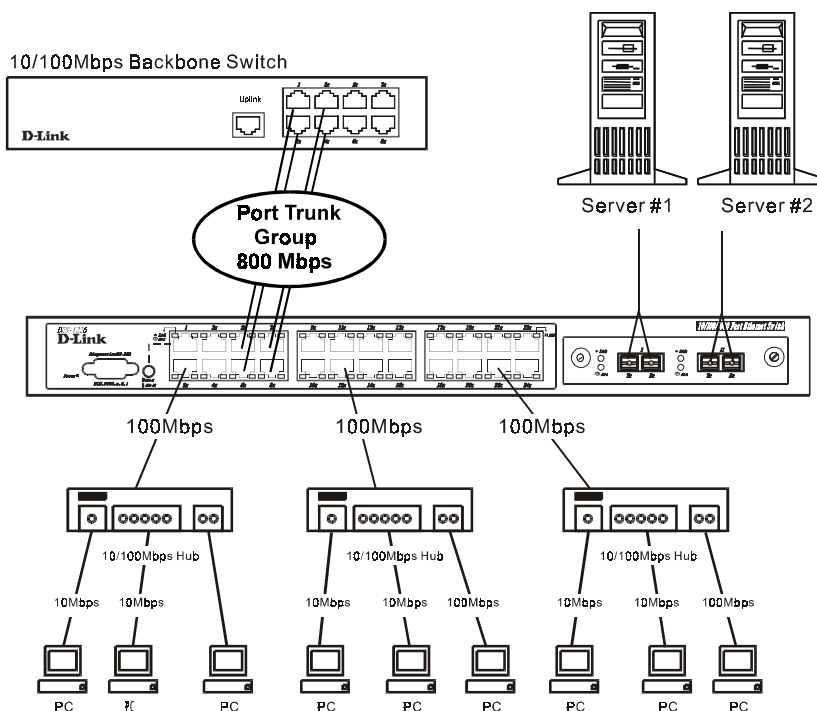
Figure 5-4 Example of Port Trunk Group
