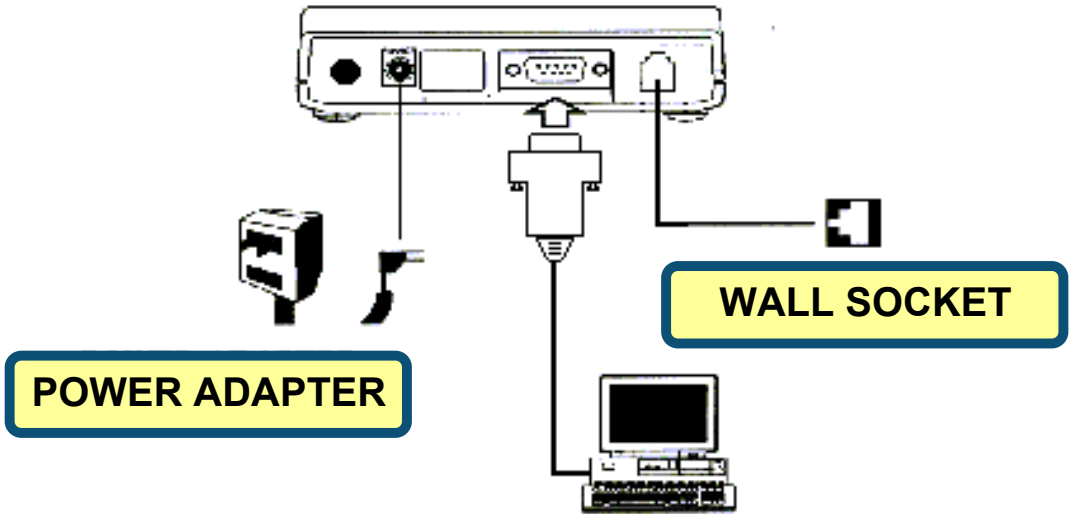
External Modem Diagram
